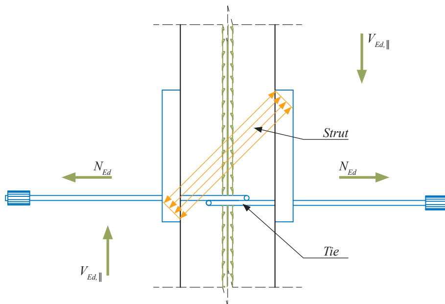
Figure 3. Strut-and-tie model for transverse shear load transfer.
