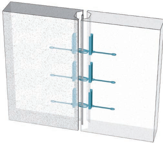
Figure 1. PVL® Connecting Loops in the joint of wall panels.
