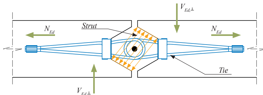
Figure 3. Strut-and-tie model for transverse shear load transfer.
