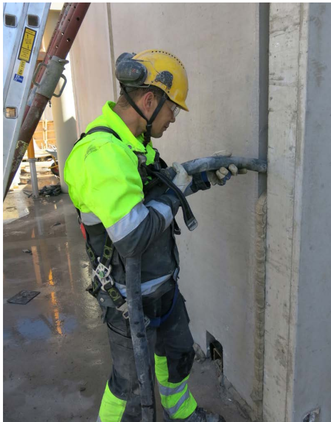
Figure 23. Casting of the joint.
